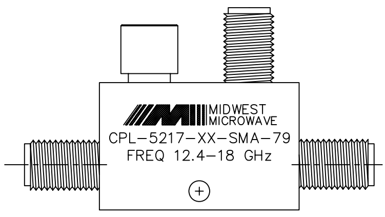
BACKSIDE MARKING
