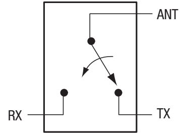
Figure 1. SKY13314-374LF Block Diagram
