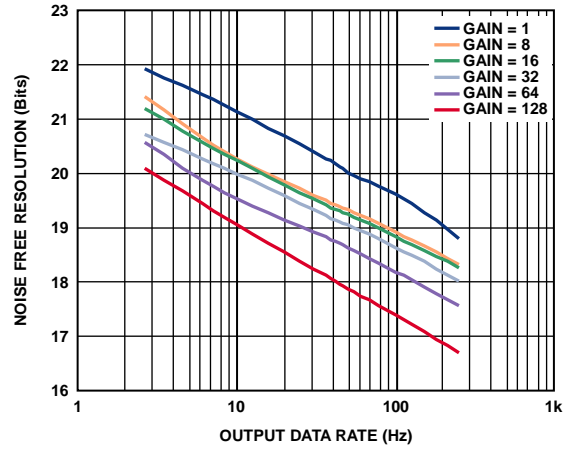
Figure 21. Noise Free Resolution in Fast Settling Mode ( V_{REF} = 5 V , Averaging by 16, Sinc^4 Filter, Chop Disabled)
