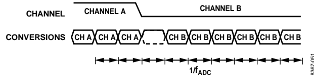
Figure 55. Fast Settling, Sinc 4 Filter
