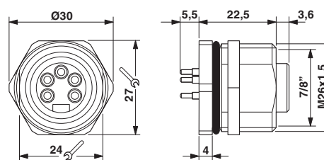
7/8" flush-type socket
