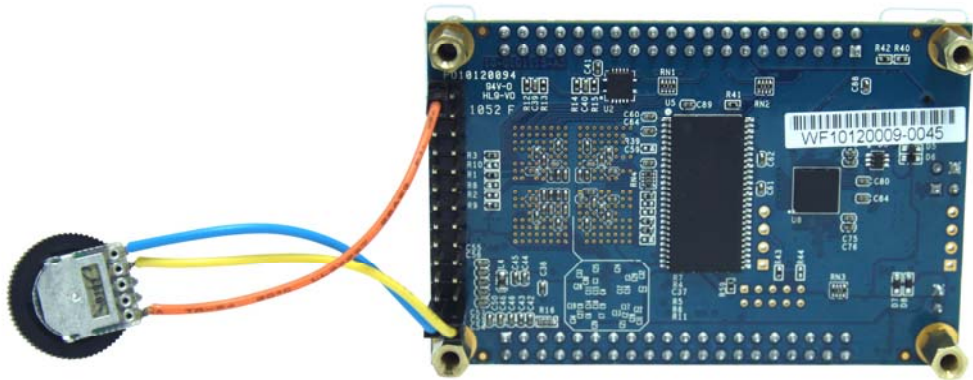
Figure 8-5 ADC Reading hardware setup
