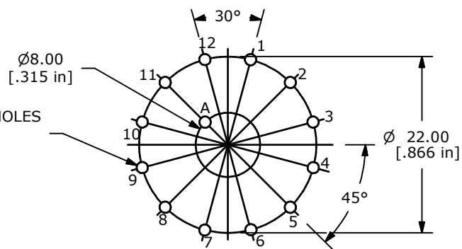
P.C.B MOUNTING PLATE
