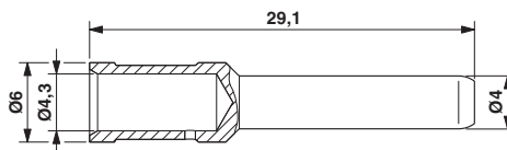
Dimensioned drawing
