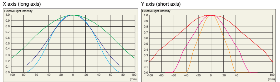
Wide Area Model (FL-BR9120W)
